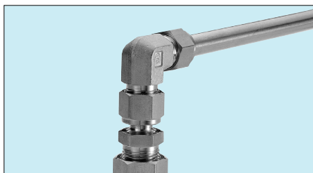
4. Connect union elbow to male adapter by tightening the Hy-Lok nut while keeping the elbow in the desired direction. Then install the tubing into the other end of elbow.
