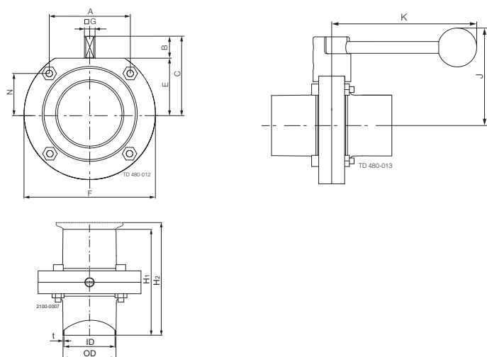
Fig. 1. Dimensions - valve.
