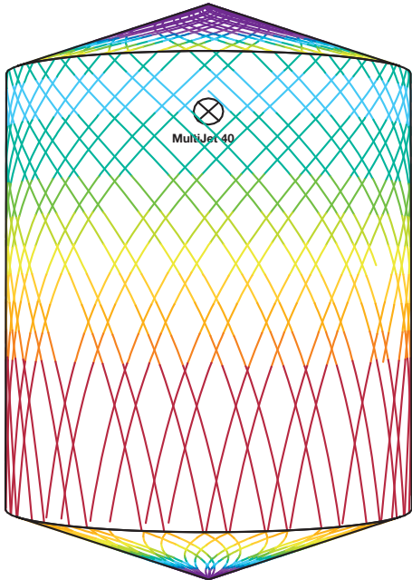
D5m H6m, Toftejorg MultiJet 40, 4 x ø6 mm, 100% Time = 4.3 min., Water consumption = 887 l
