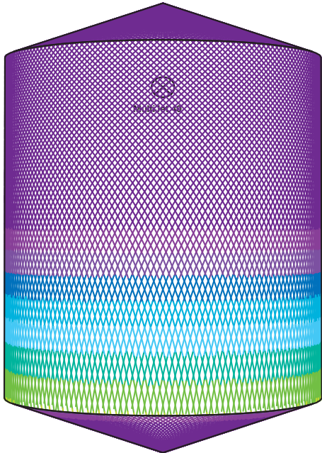
D5m H6m, Toftejorg MultiJet 40, 4 x ø6 mm, 100% Time = 18.2 min., Water consumption = 3760 l
